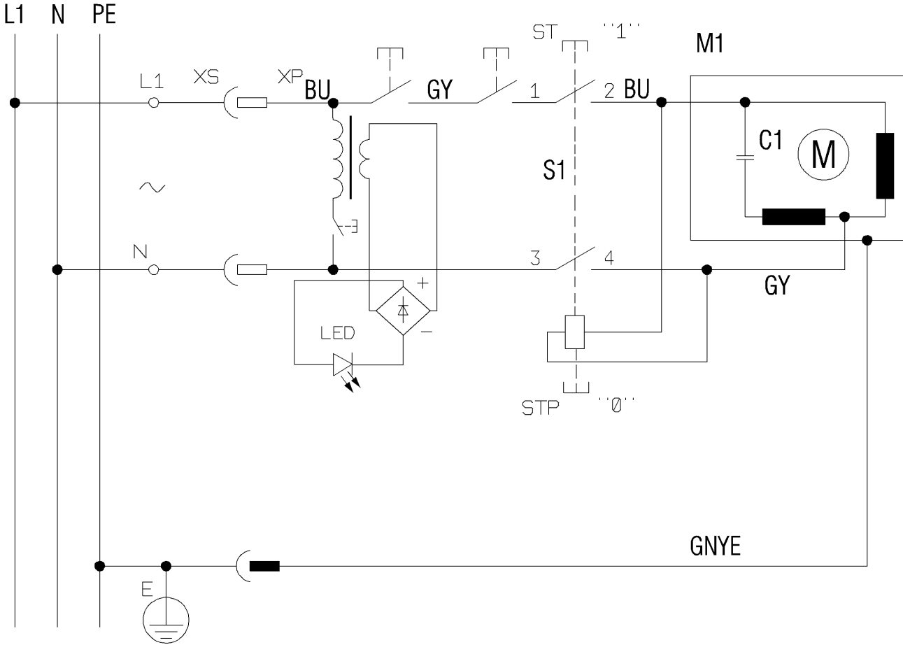
M1: induction motor 220-240V / 50Hz S1: KJD6 C1: 12μF
